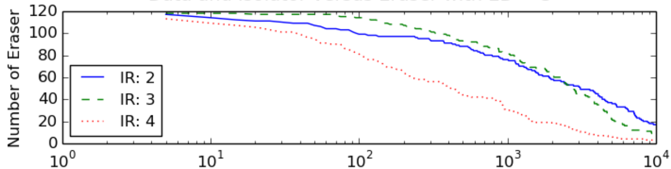
Data and Isolator versus Eraser with ED = 3
