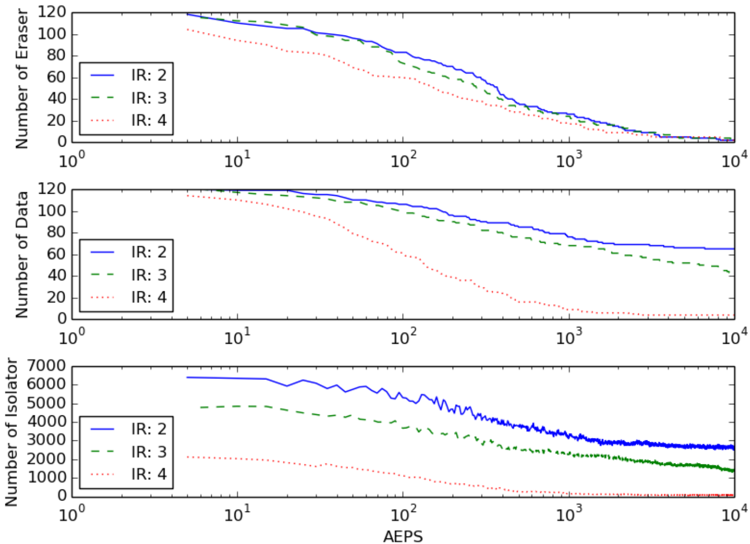
Data and Isolator versus Eraser with ED = 4
