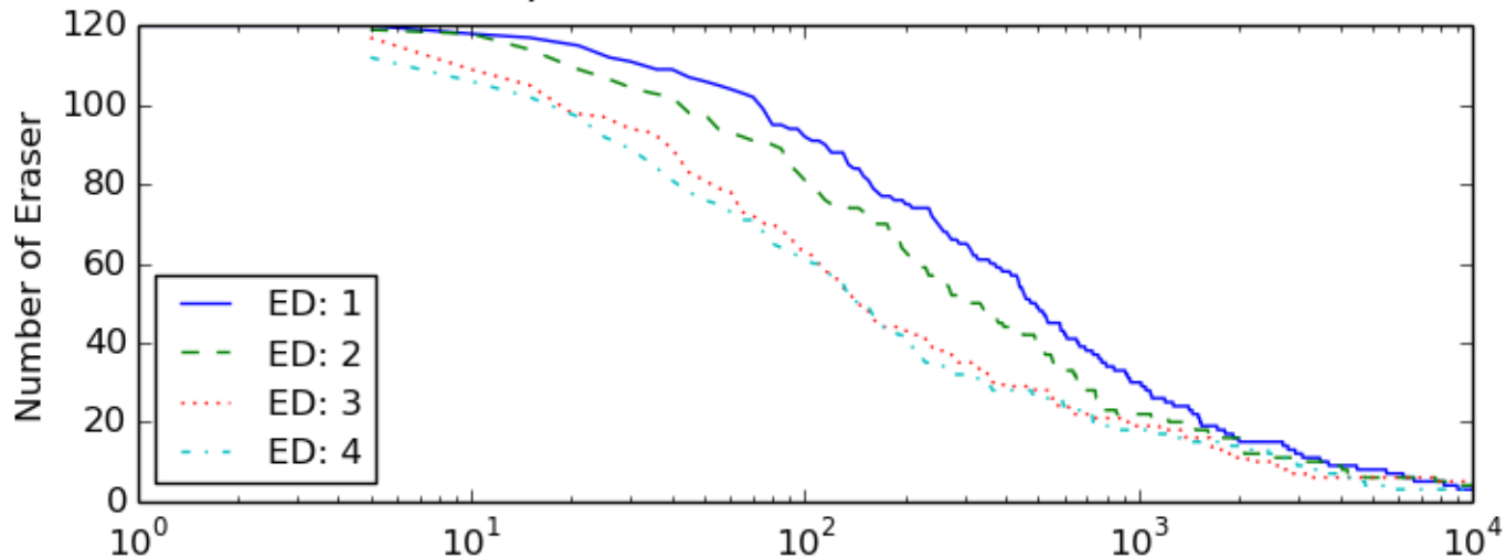
Population of Eraser and Data
