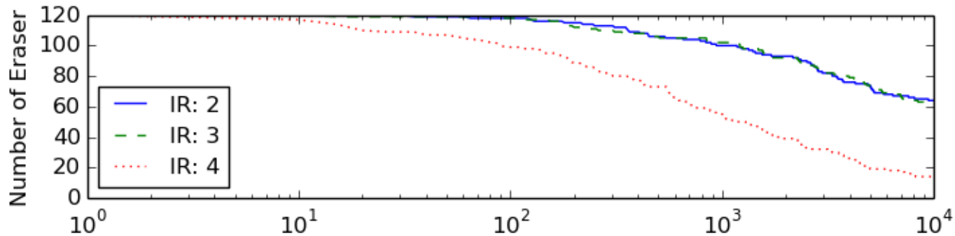
Data and Isolator versus Eraser with ED = 1
