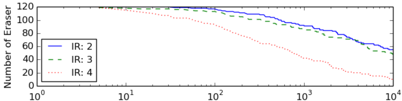
Data and Isolator versus Eraser with ED = 2
